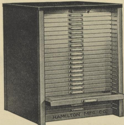
No. 12435 (Steel) No. 2435 (Wood) Floor Space, 35 x 21 5/8". Height, 43".
