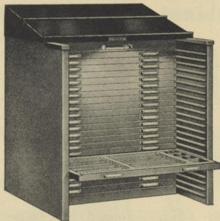
No. 12437 (Steel) Floor Space, 43 3/4 x 30 1/4". Height at front, 40".
